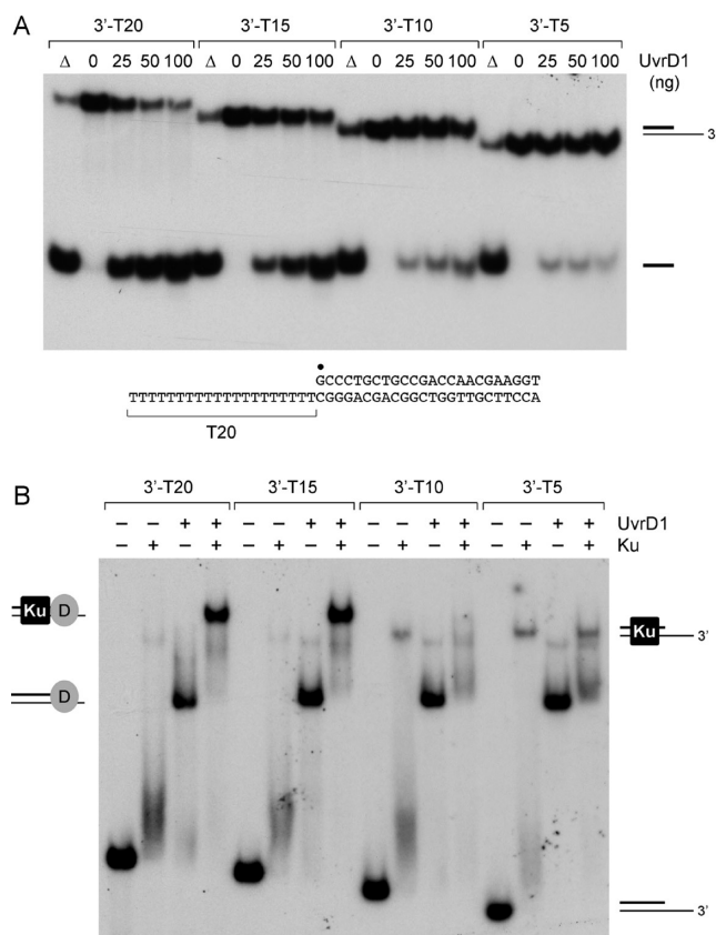
FIGURE 7: Effect of 3' tail length on helicase activity and DNA binding. (A) Helicase reaction mixtures contained 50 nM duplex DNA substrate with 3'-T20, 3'-T15, 3'-T10, or 3'-T5 tails, 1 mM ATP, 75 ng of Ku, and 0, 25, 50, or 100 ng of UvrD1. The products were analyzed by native PAGE and visualized by autoradiography. A control reaction lacking enzyme that was heat denatured prior to PAGE is shown in lane \Delta . The 3'-T20 substrate is shown at the bottom with the 5'- ^{32} P label denoted by \bullet . (B) DNA-binding reaction mixtures contained 0.5 pmol of ^{32} P-labeled 3'-tailed DNAs as specified, 100 ng of UvrD1 (where indicated by +), and 75 ng of Ku (where indicated by +). The products were analyzed by native gel electrophoresis. The free DNAs and various protein–DNA complexes (depicted at left and right) were visualized by autoradiography.
