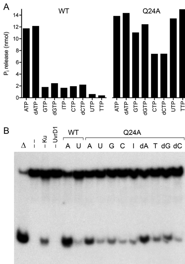
FIGURE 5: Role of the Q motif (Gln24) in NTP substrate specificity. (A) Phosphohydrolase reaction mixtures contained 1 mM indicated ribonucleoside or deoxyribonucleoside triphosphate and either 50 ng of wild-type UvrD1 or 200 ng of the Q24A mutant. The extents of phosphate production are shown. (B) Complete helicase reaction mixtures contained 50 nM ^{32} P-labeled tailed duplex DNA substrate, 75 ng of Ku, 100 ng of wild-type UvrD1 or Q24A, and 1 mM indicated NTP or dNTP. The products were analyzed by native PAGE and visualized by autoradiography. Reactions without added protein (lane –), with wild-type UvrD1 only (–Ku), or with Ku only (–UvrD1) were included as controls. A reaction mixture lacking protein that was heat denatured prior to PAGE is shown in lane Δ.
