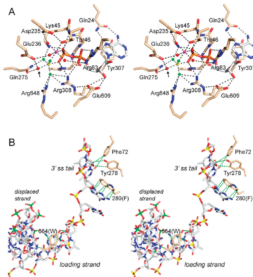
FIGURE 2: ATPase active site and DNA contacts. (A) Stereoview of the phosphohydrolase active site of DNA-bound E. coli UvrD (PDB 2IS6) as a transition state mimetic in complex with Mg 2+ (magenta sphere), ADP (stick model with gray carbons), and a trigonal planar MgF 3 (depicted with the magnesium as a yellow sphere and the fluorines as green spheres). Waters are rendered as red spheres. The putative water nucleophile located apical to the leaving \beta -phosphate oxygen is indicated by an arrow. The atomic contacts of the conserved active site residues (stick models with beige carbons) are denoted by dashed lines. The residue numbers refer to the equivalent side chains in UvrD1 that were subjected to alanine scanning. (B) Stereoview of DNA contacts in the crystal structure of E. coli UvrD bound to a 3'-tailed duplex DNA (from PDB 2IS6). The 3'-tailed strand (the loading strand for initial helicase binding, on which the enzyme translocates 3' to 5') is depicted as a stick model with phosphorus atoms colored yellow. The complementary strand that forms the duplex segment (the displaced strand unwound by helicase translocation) is depicted with phosphorus atoms in green. Conserved aromatic residues that make base stacking and van der Waals contacts with the DNA (green dashed lines) are shown, with residue numbering referring to the equivalents in UvrD1.
