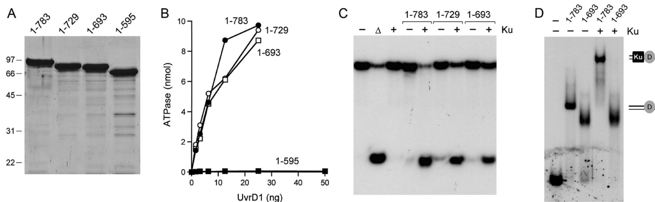
FIGURE 6: Effects of C-terminal deletions. (A) Aliquots (5 \mu g) of full-length UvrD1-(1–783) and the C-terminal truncation mutants UvrD1-(1–729), UvrD1-(1–693), and UvrD1-(1–595) were analyzed by SDS–PAGE. The Coomassie blue-stained gel is shown. The sizes (kDa) and positions of marker proteins are indicated on the left. (B) ATPase assays were performed as described in Experimental Procedures. ^{32} P i release from 1 mM [ \gamma - ^{32} P]ATP is plotted as a function of input UvrD1 for each enzyme assayed. (C) Complete helicase reaction mixtures contained 1 mM ATP, 50 nM ^{32} P-labeled tailed duplex DNA substrate, 75 ng of Ku (where indicated by +), and 100 ng of UvrD1 protein as specified. The products were analyzed by native PAGE and visualized by autoradiography. A reaction lacking protein that was heat denatured prior to PAGE is shown in lane \Delta . (D) DNA-binding reaction mixtures contained 0.5 pmol of ^{32} P-labeled 3'-tailed DNA, 100 ng of UvrD1-(1–783) or UvrD1-(1–693), and 75 ng of Ku (where indicated by +). The free DNA and protein–DNA complexes (depicted on the right) were resolved by native PAGE and visualized by autoradiography.
