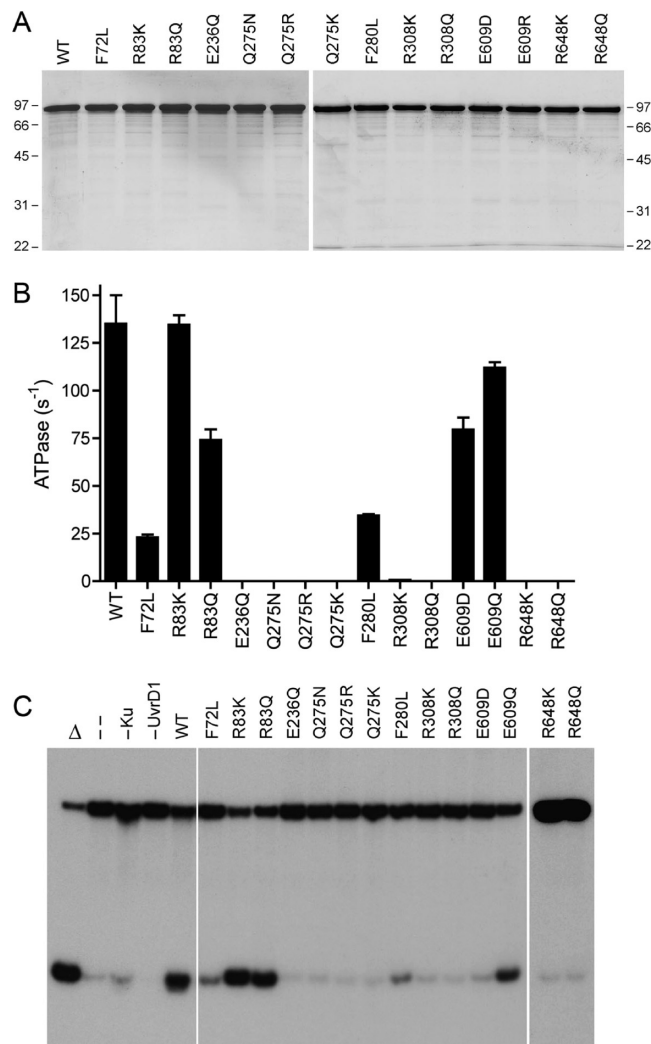
FIGURE 4: Effects of conservative mutations on UvrD1 activities. (A) Aliquots (3 \mu\text{g} ) of recombinant wild-type (WT) UvrD1 and the indicated mutants were analyzed by SDS–PAGE. The Coomassie blue-stained gels are shown. The sizes (kDa) and positions of marker proteins are indicated. (B) ATPase specific activity was determined as specified under Experimental Procedures. Each datum is the average of three separate UvrD1 titration experiments; error bars denote the standard deviation. (C) Helicase reactions were performed as described under Experimental Procedures. Complete reaction mixtures contained 1 mM ATP, 50 nM ^{32}\text{P} -labeled tailed duplex DNA substrate, 75 ng of Ku, and 100 ng of wild-type or mutant UvrD1 protein as specified. The products were analyzed by native PAGE and visualized by autoradiography. Reactions without added protein (lane \Delta ), with wild-type UvrD1 only ( -\text{Ku} ), or with Ku only ( -\text{UvrD1} ) were included as controls. A reaction lacking protein that was heat denatured prior to PAGE is shown in lane \Delta .
