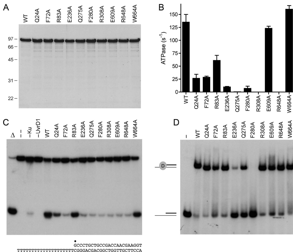
FIGURE 3: Effects of alanine mutations on UvrD1 activities. (A) Aliquots (5 \mu g) of recombinant wild-type (WT) UvrD1 and the indicated Ala mutants were analyzed by SDS-PAGE. The Coomassie blue-stained gel is shown. The sizes (kDa) and positions of marker proteins are indicated on the left. (B) ATPase specific activity was determined as specified under Experimental Procedures. Each datum is the average of two separate UvrD1 titration experiments; error bars denote the mean absolute error. (C) Helicase reactions were performed as described under Experimental Procedures. Complete reaction mixtures contained 1 mM ATP, 50 nM 32 P-labeled tailed duplex DNA substrate, 75 ng of Ku, and 100 ng of wild-type or mutant UvrD1 protein as specified. The products were analyzed by native PAGE and visualized by autoradiography. Reactions without added protein (lane -), with wild-type UvrD1 only (-Ku), or with Ku only (-UvrD1) were included as controls. A reaction lacking protein that was heat denatured prior to PAGE is shown in lane Δ. The 3'-tailed duplex helicase substrate is shown at the bottom with the 5'- 32 P label denoted by ●. (D) Binding of UvrD1 to the helicase substrate. Binding reactions were performed as described under Experimental Procedures. Complete reaction mixtures contained 1 pmol of 32 P-labeled tailed duplex DNA substrate and 100 ng of wild-type or mutant UvrD1 protein as specified. UvrD1 was omitted from the control reaction in lane -. The products were analyzed by native PAGE and visualized by autoradiography. The positions of the free DNA and the UvrD1-DNA complex are indicated on the left.
